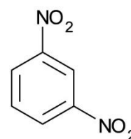
2. 1,3-Dinitrobenzene
