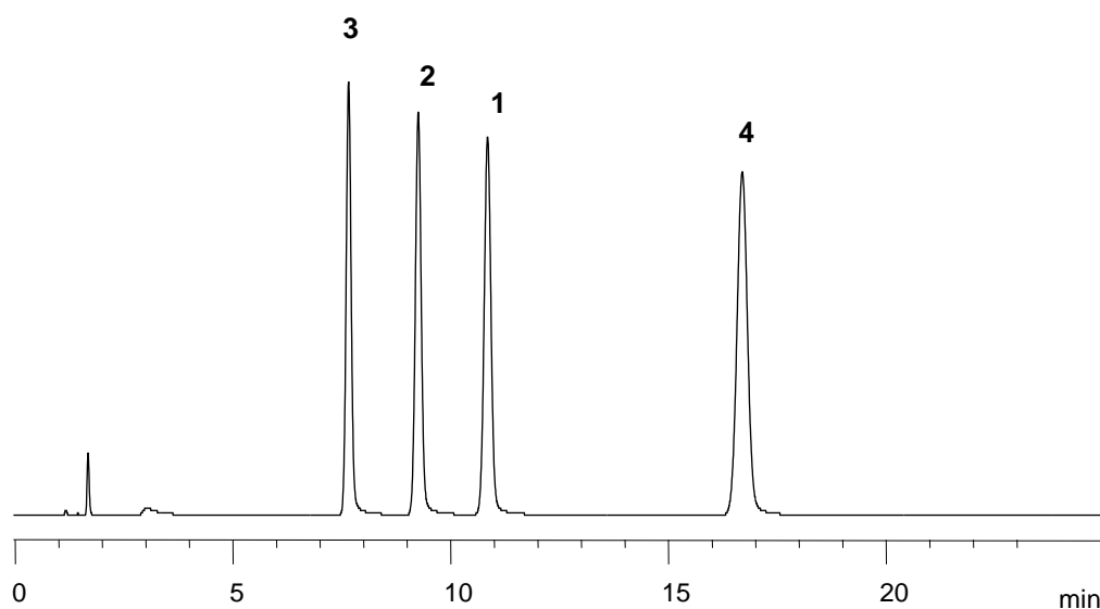
2. 1,3-Dinitrobenzene
