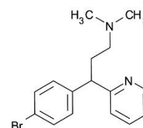
2. Brompheniramine
