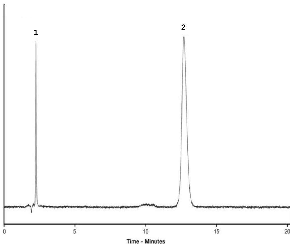
2. Brompheniramine
