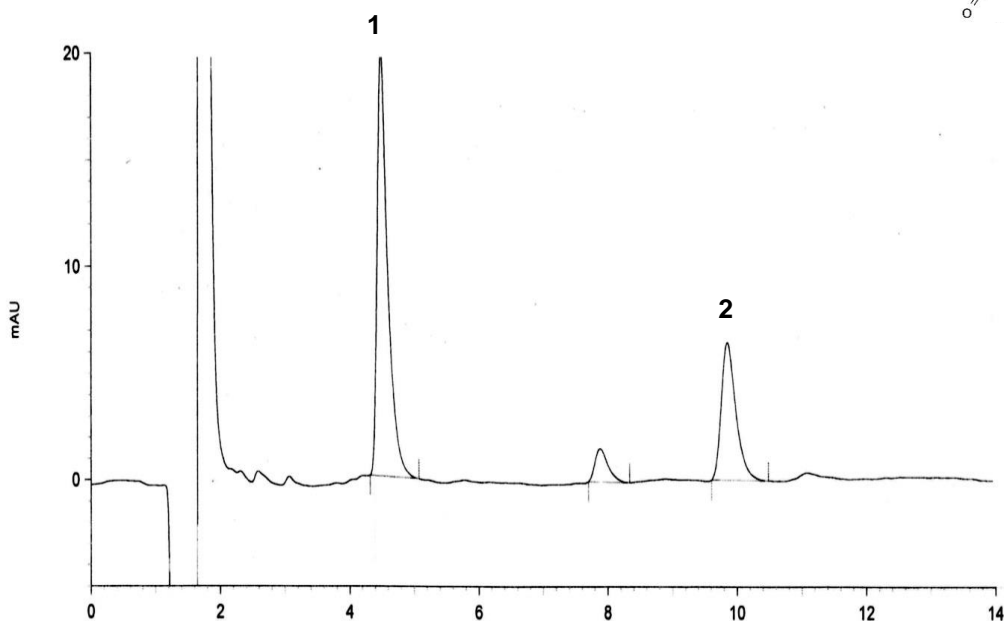
1. DOTATATE
