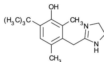
1. Oxymetazoline
