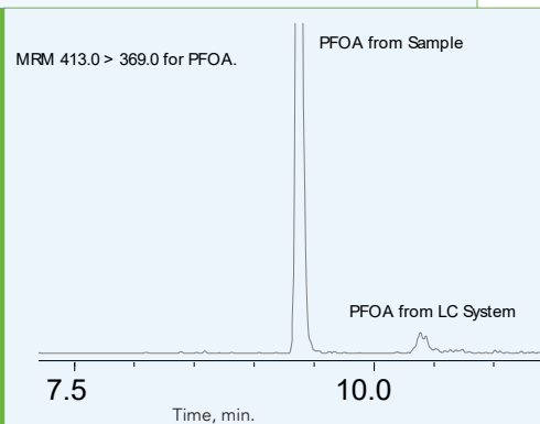
Figure 4. PFOA from sample and LC system run on a HALO® PFAS Delay column and a HALO® PFAS column.
