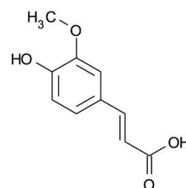
3. Ferulic acid
