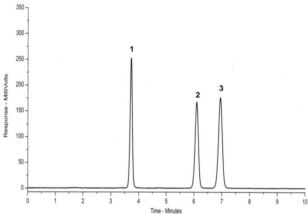
2. p-Coumaric acid
