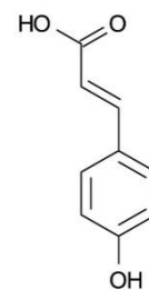
2. p-Coumaric acid
