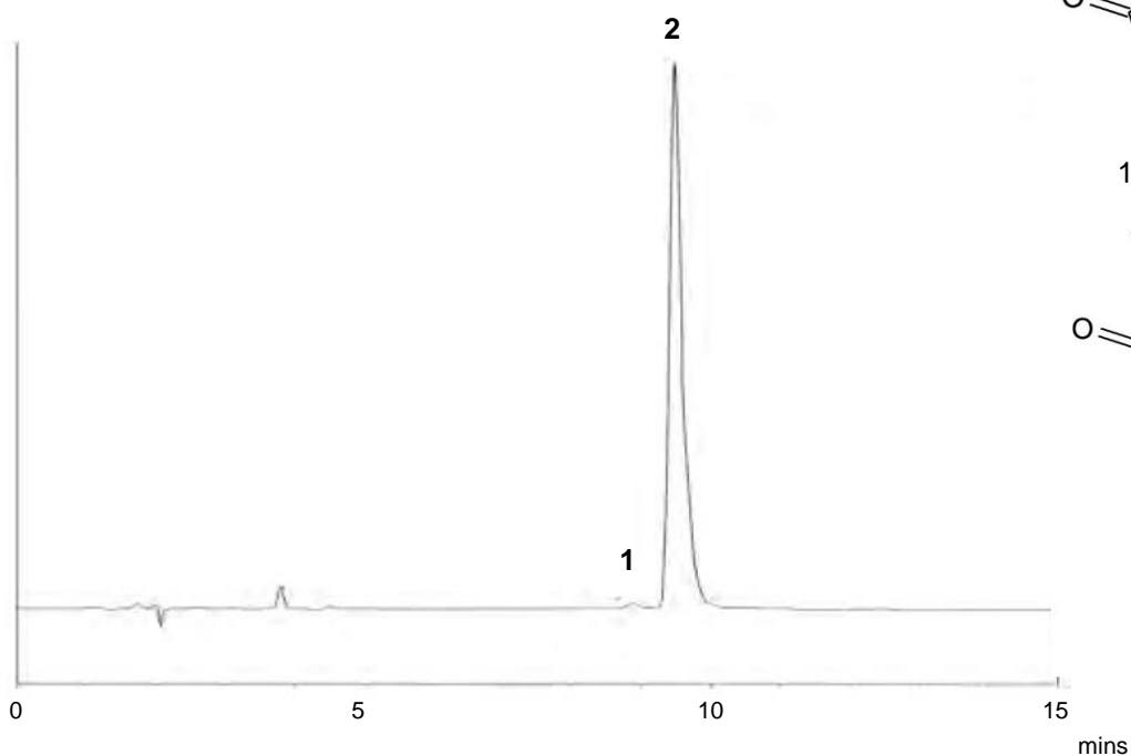
2. Pilocarpine
