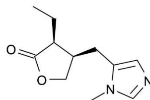
2. Pilocarpine
