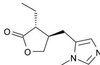
1. Isopilocarpine
